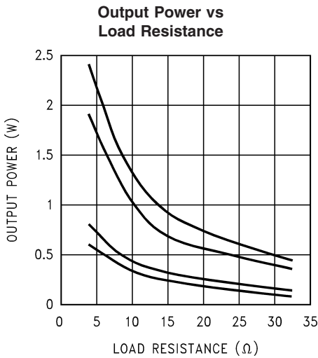
201163C0 f_{IN} = 1kHz, at (from top to bottom at 20\Omega ): V_{DD} = 5V, THD = 10\%; V_{DD} = 5V, THD = 1\%; V_{DD} = 3V, THD = 10\%; V_{DD} = 3V, THD = 1\%
